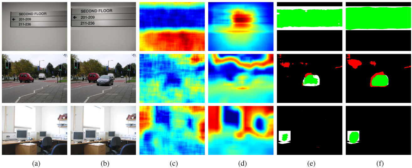
Fig. 3: Forgery detection results for scaling (the first row), copy-and-move (the second row) and cut-and-paste (the third row) forgery. (a) Original image, (b) forged image, (c) predicted correlation field, (d) actual correlation field, (e) detection result by CFAR and (f) refined detection result by our proposed algorithm.
