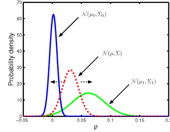
Fig. 2: How the correlation distribution changes as the sliding window moves across the boundary region.
